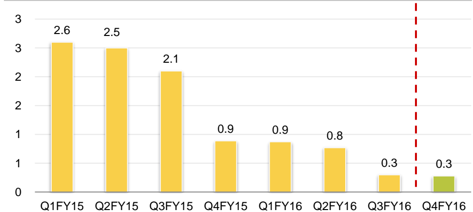
Gross NPA (%)
